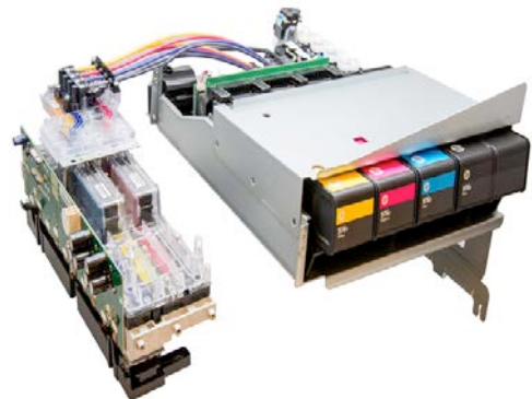
Figure 6. Off-axis PageWide writing engine assembly
