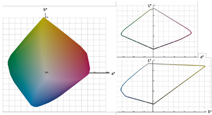
Figure 3. Color gamut of HP PageWide XL Pigment Inks on HP Heavyweight Coated Paper
