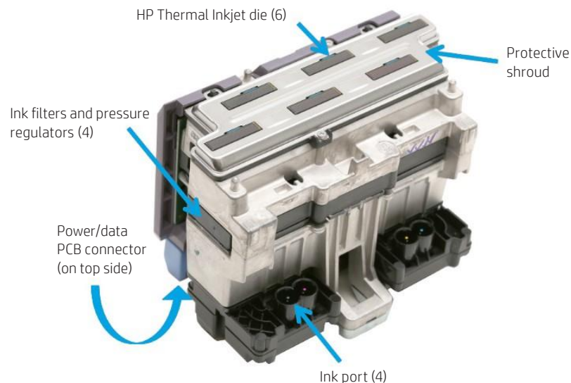
Figure 1. HP 841 Printhead used in HP PageWide XL printers
