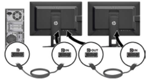
HP Z Display Daisy-chaining
