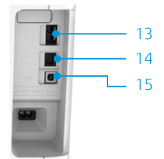
Rear I/O panel close-up
