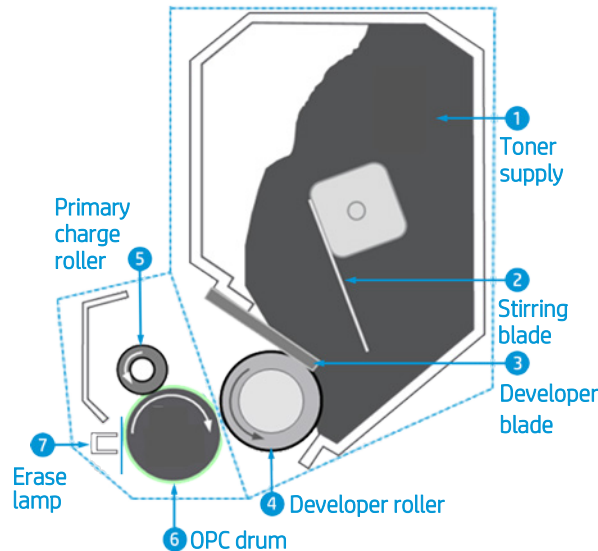
Two-part cartridge system made of imaging drum cartridge and toner supply cartridge
