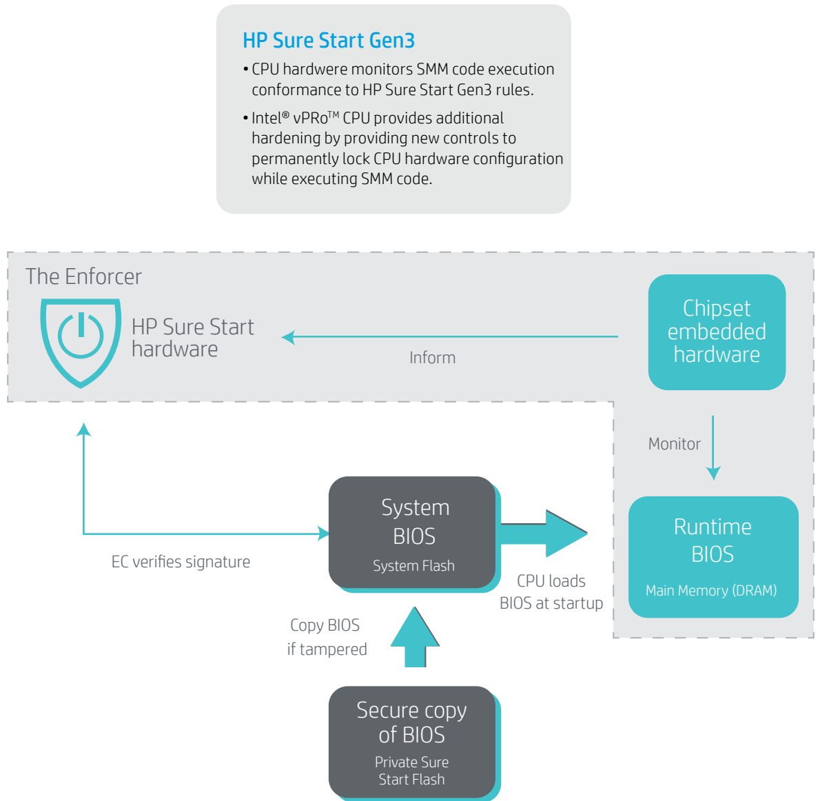
Figure 2 Runtime Intrusion Detection architecture (applies to HP Elite products equipped with 7th generation Intel® Core™ processors and higher)
