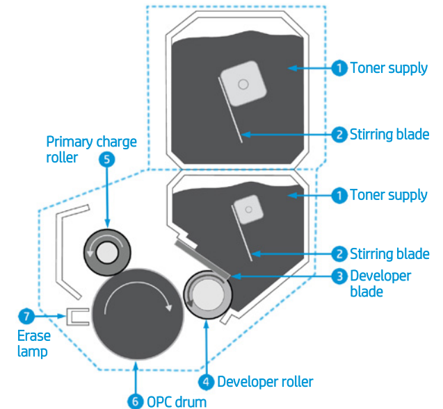
Two-part cartridge system consisting of process cartridge (imaging drum and developer) and toner supply cartridge
