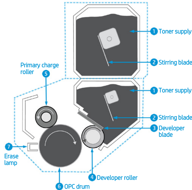
Two-part cartridge system consisting of process cartridge (imaging drum and developer) and toner supply cartridge
