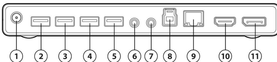
HP 3005pr USB3 Port Replicator (Y4H06AA) back view
